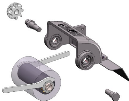
Fig. 13: Changing the wire brush
