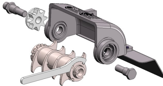
Fig. 14: Replacing knives
