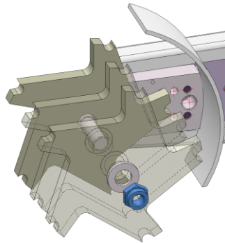
Fig. 12: Replacing knives on the groove cutter
