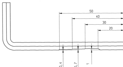
Fig. 8: Allen wrench with notches
